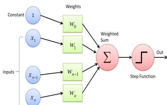
Fig. 4 Perceptron neural network
